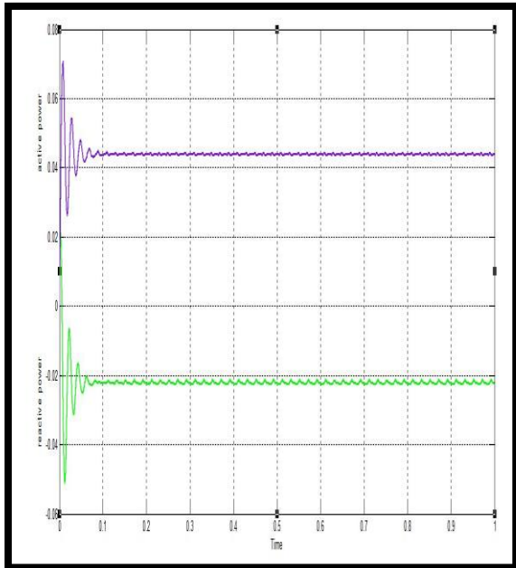
Figure 6.10 Active and Reactive Power at Source Side
