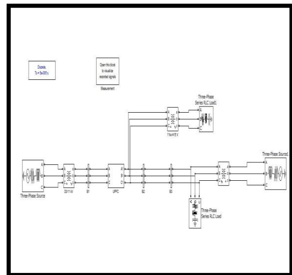
Figure 6.1 Three phase compensated network connect with UPFC system
