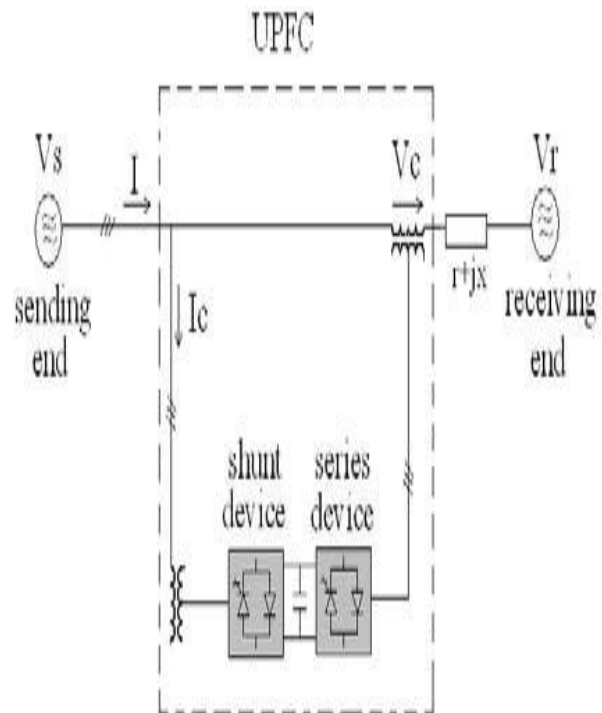
Figure 4.2 UPFC Set up Scheme
