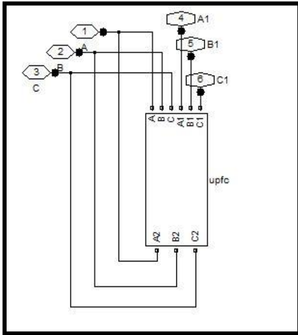
Figure 6.2 UPFC Subsystem
