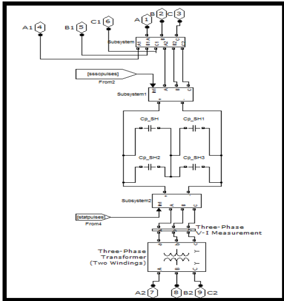
Figure 6.6 Controlling Subsystem
