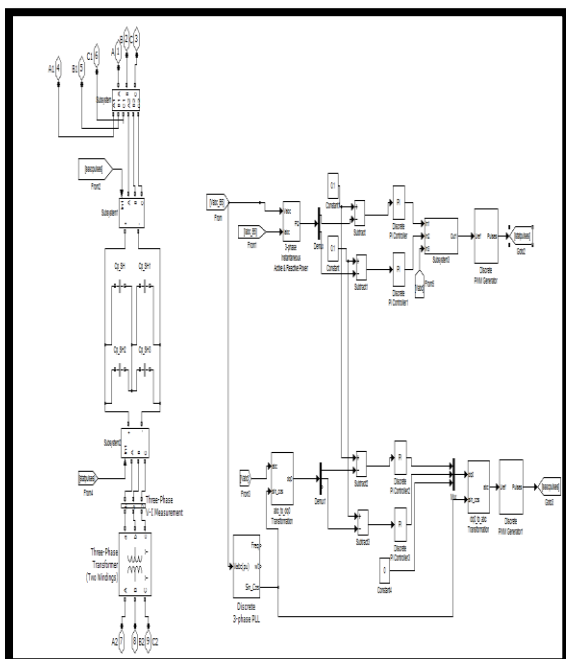
Figure 6.3 Configuration of UPFC System
