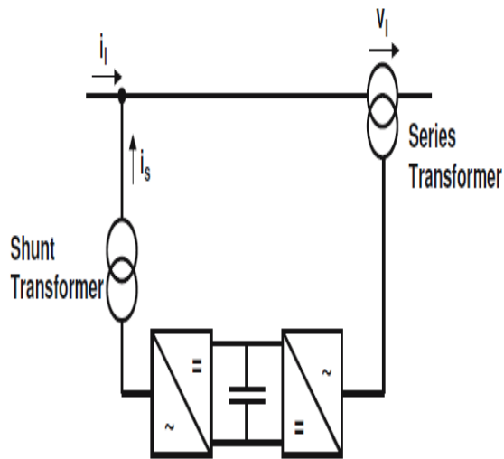
Figure 4.1 Principle configuration of an UPFC
