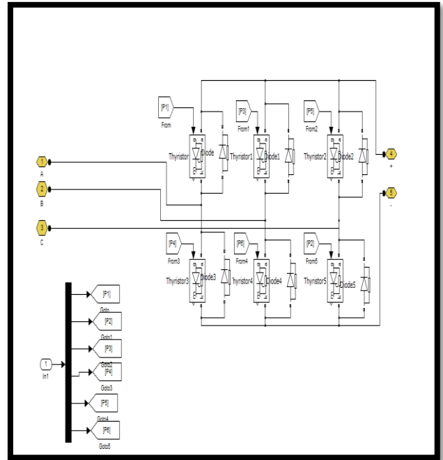
Figure 6.4 VSC configuration in UPFC design
