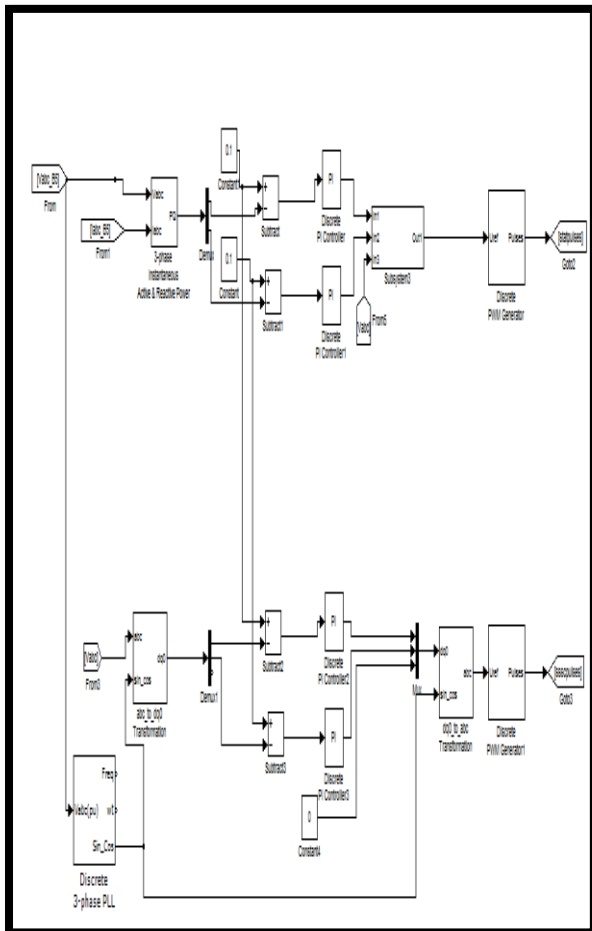
Figure 6.5 Control Strategy of UPFC System
