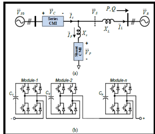
Figure 5.2 New transformer-less UPFC, (a) System Configuration of Transformer-less UPFC, (b) One phase of the cascaded multilevel inverter
